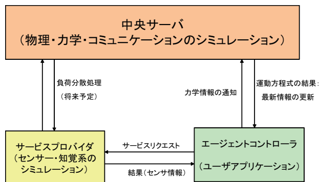
Fig.3 Software configuration of SIGVerse
